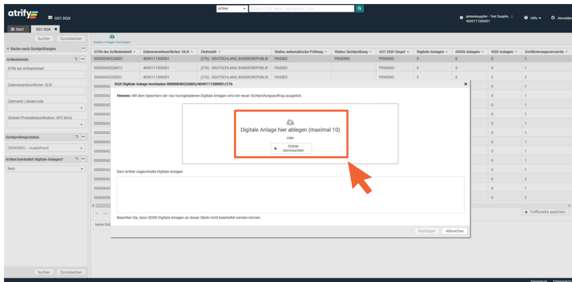
Abbildung 2 – 7: Upload Dialog
