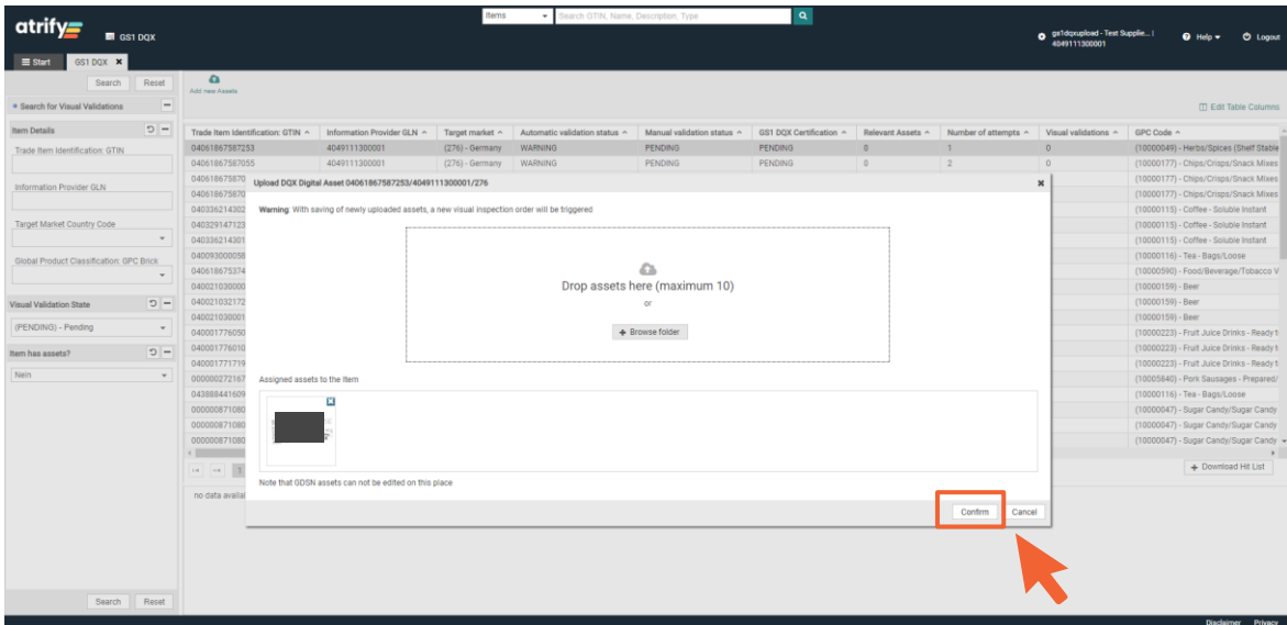
Figure 2 - 9: Confirm upload
