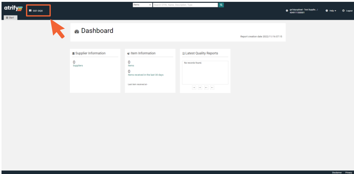
Figure 2 - 1: Dashboard
