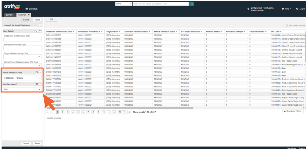
Figure 2 - 5: Set filter
