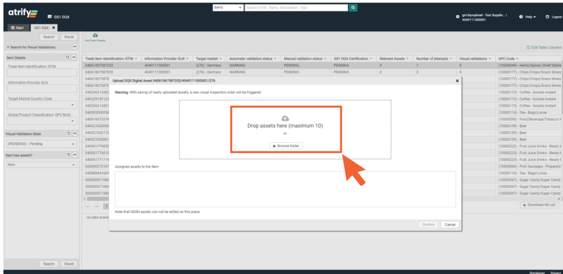
Figure 2 - 7: Upload dialog
